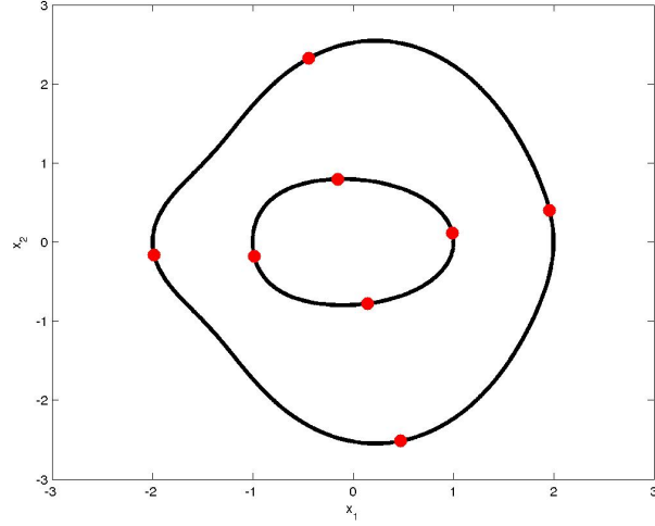
Fig. 3. The determinantal quartic curve of Example 12 (black) and eight of its points (red) as returned by RealDet.
