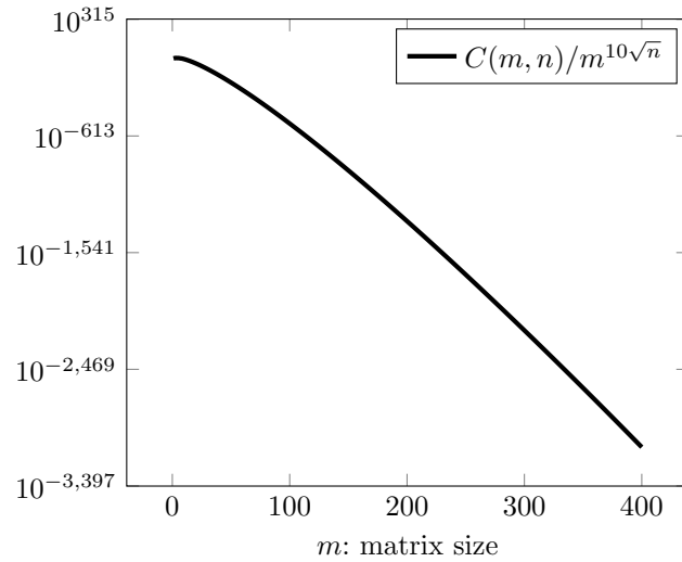
Fig. 6. Complexity bound for n = m^2 .
