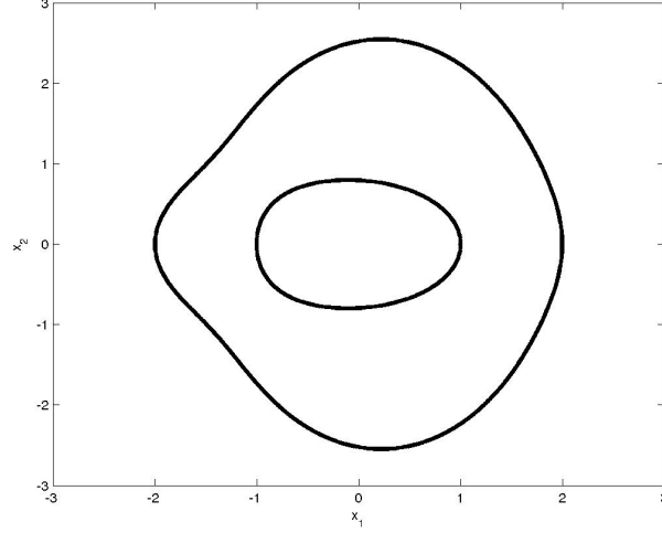
Fig. 2. The smooth quartic curve of Example 12 with its two nested ovals.
