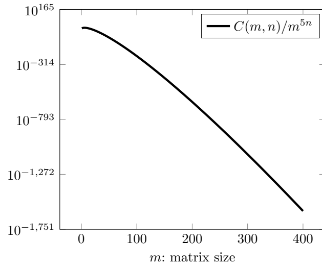
Fig. 7. Complexity bound for n = \frac{m^2+m}{2} .
