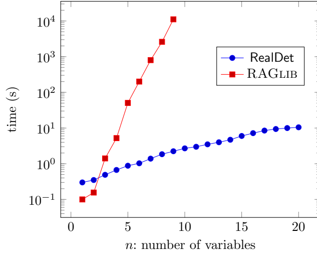
Fig. 4. Timings for m = 3 and n \leq 20
