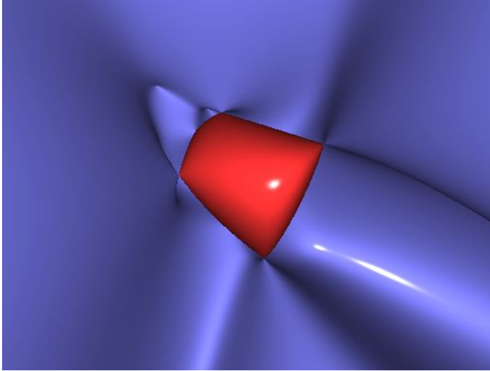
Fig. 1. A spectrahedron (red) with its real determinantal variety.
