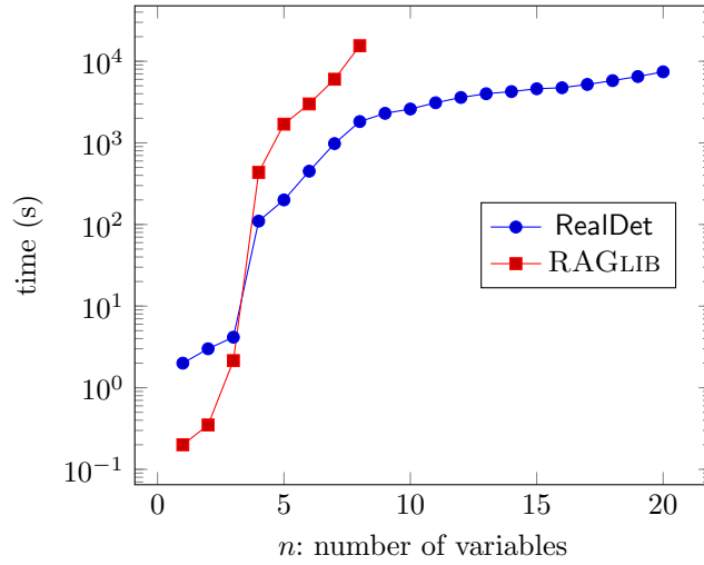
Fig. 5. Timings for m = 4 and n \leq 20
